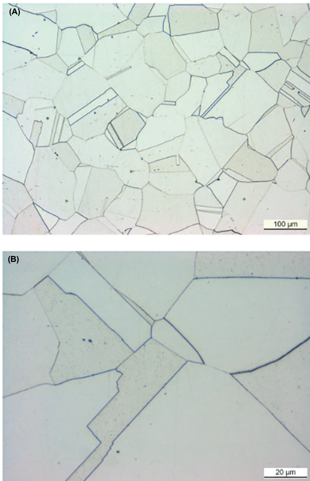
Figure A.10—Acceptable Microstructure for UNS N09925, UNS N09935, UNS N09945, UNS N07716, and UNS N07725
