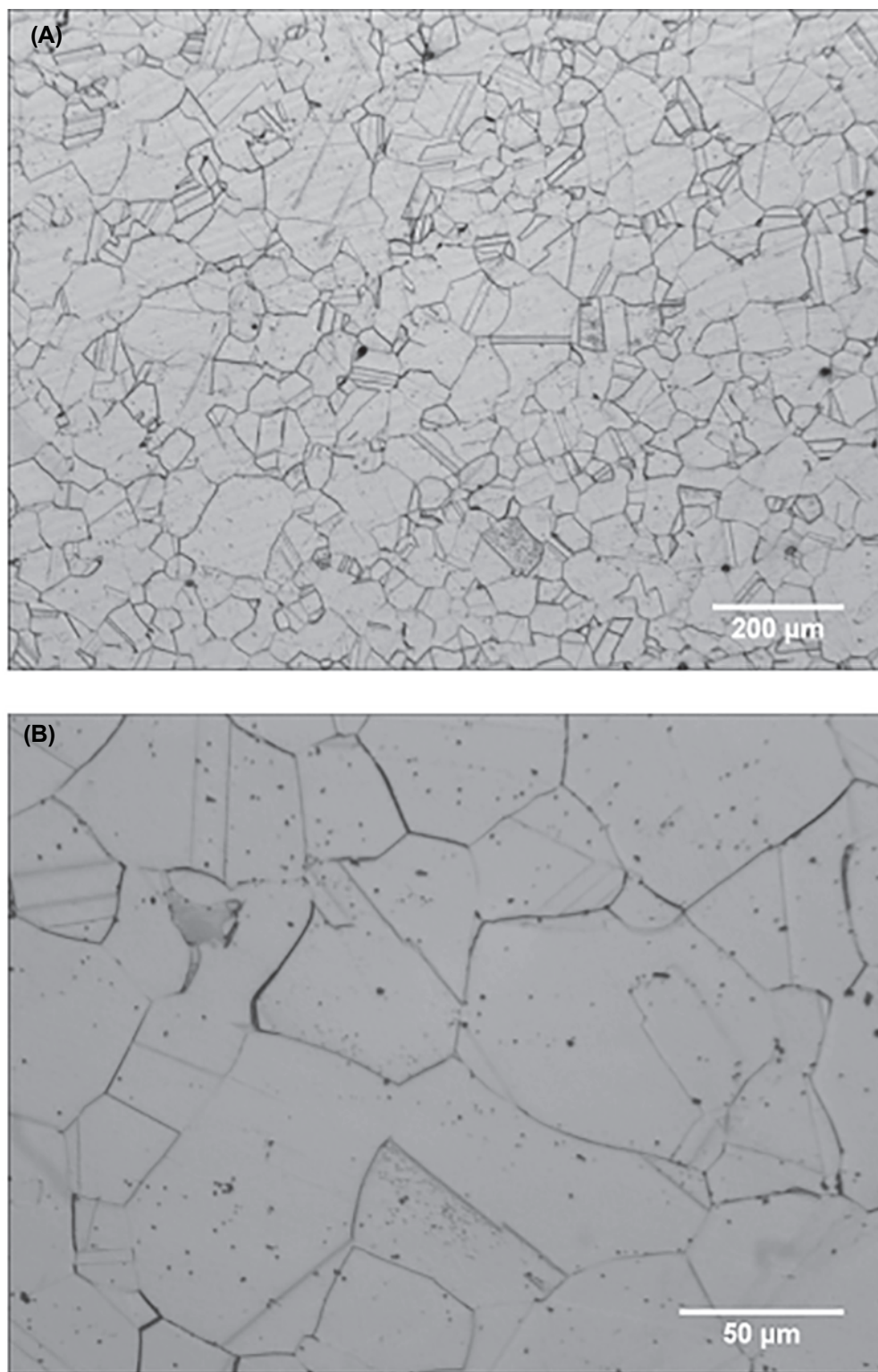
Figure A.11—Acceptable Microstructure for UNS N09925, UNS N09935, UNS N09945, UNS N07716, and UNS N07725 Showing Isolated Grain Boundary Precipitation
