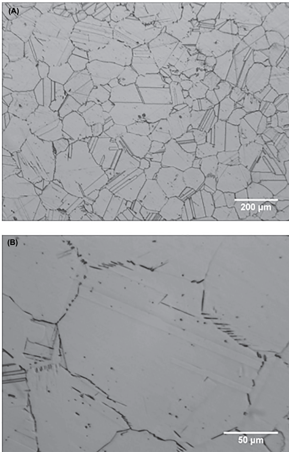
Figure A.15—Unacceptable Microstructure for UNS N09925, UNS N09935, UNS N09945, UNS N07716, and UNS N07725 Showing Acicular Grain Boundary Precipitates
