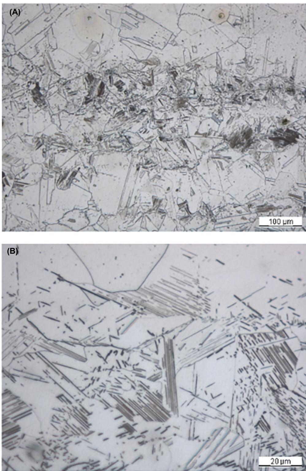
Figure A.16—Unacceptable Microstructure for UNS N09925, UNS N09935, UNS N09945, UNS N07716, and UNS N07725 Due To Acicular Precipitates
