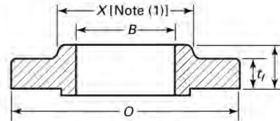
Slip-On Welding
