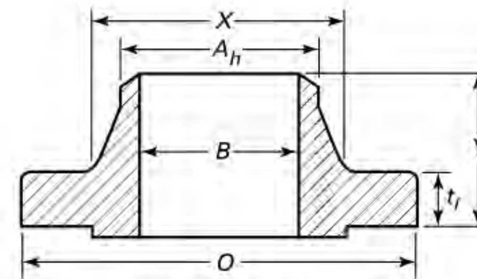
Welding Neck
