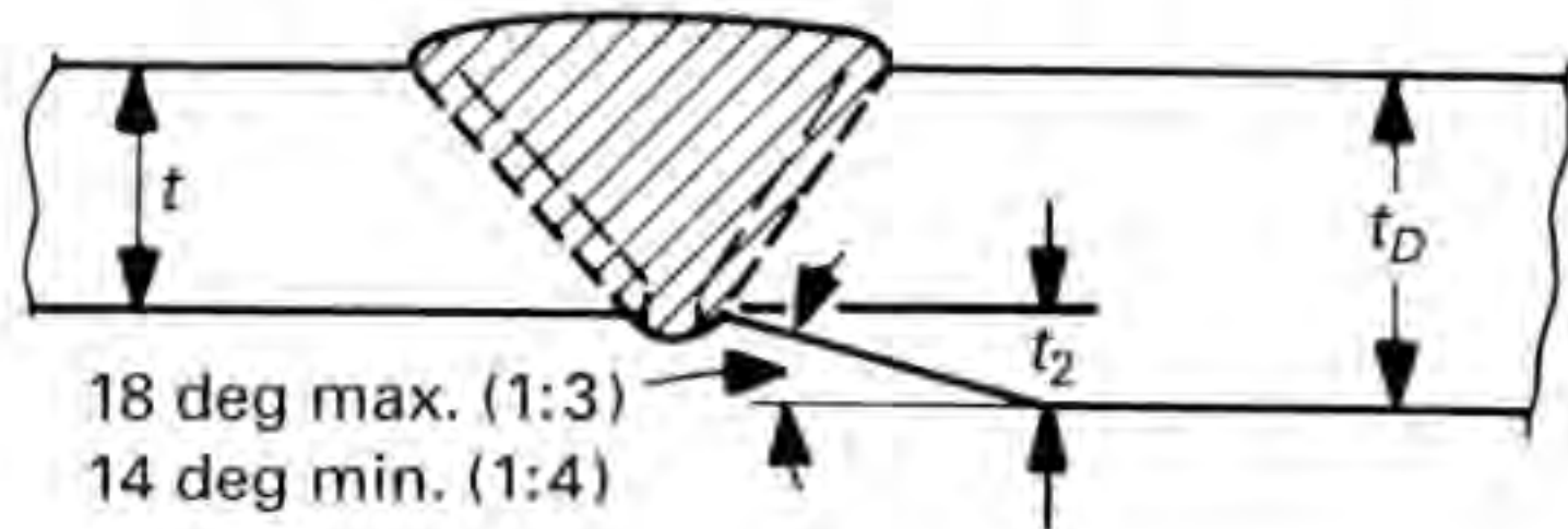
Figure 2 Bevel for Inside Thickness
