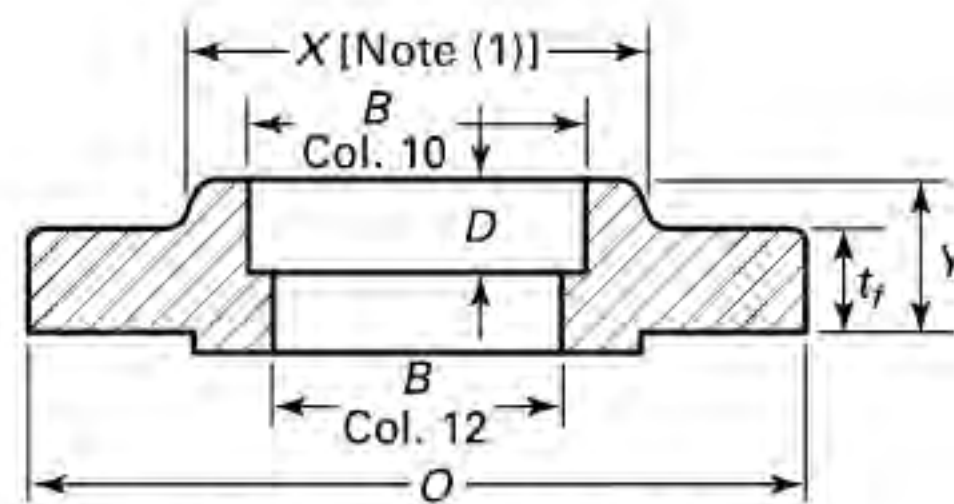
Socket Welding (NPS 1/2 to 3 Only)
