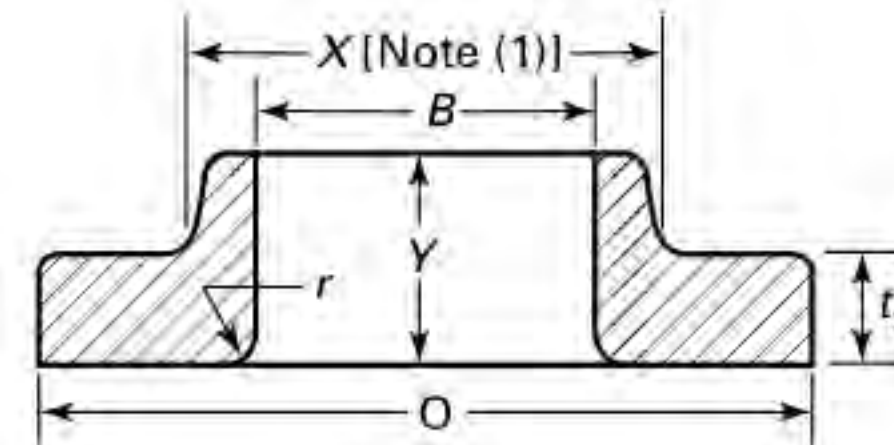
Lapped
