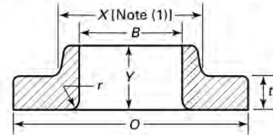
Lapped
