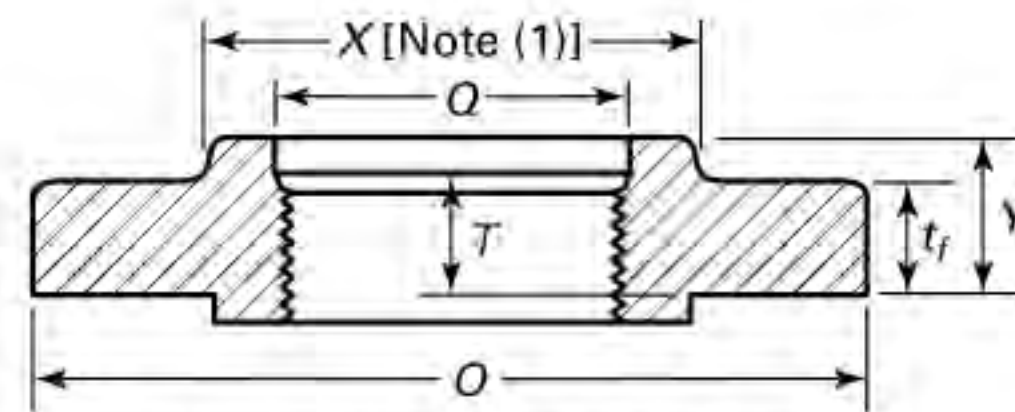
Threaded (NPS 1/2 to 2 1/2 Only)
