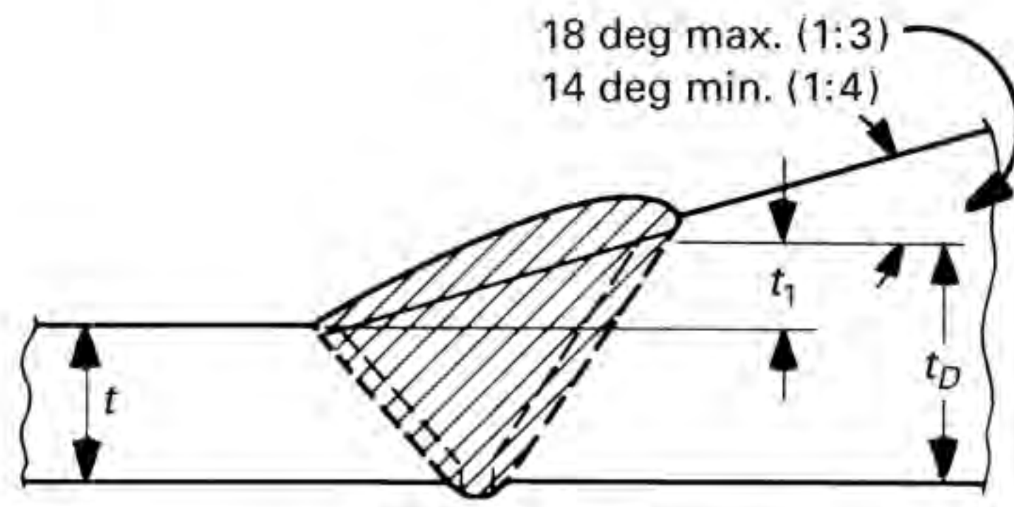
Figure 1 Bevel for Outside Thickness
