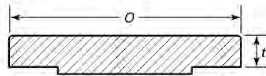
Blind
