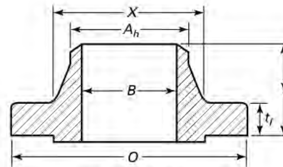
Welding Neck
