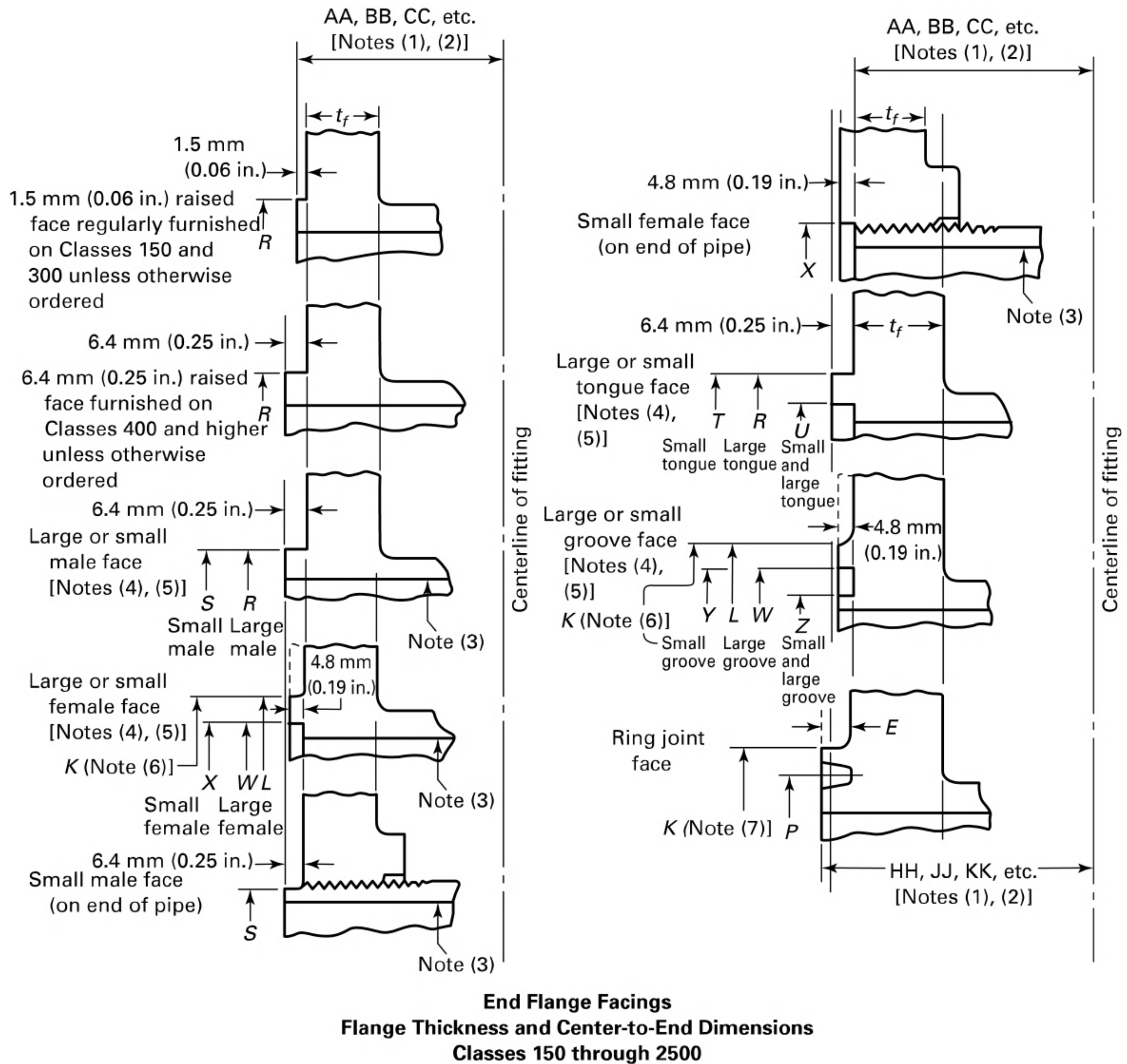
Figure 6 End Flange Facings and Their Relationship to Flange Thickness and Center-to-End and End-to-End Dimensions
