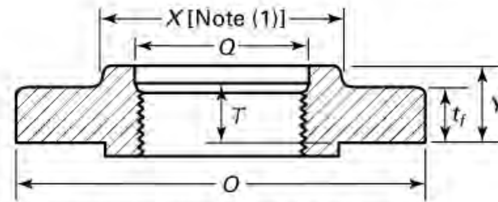
Threaded (NPS 1/2 to 2 1/2 Only)
