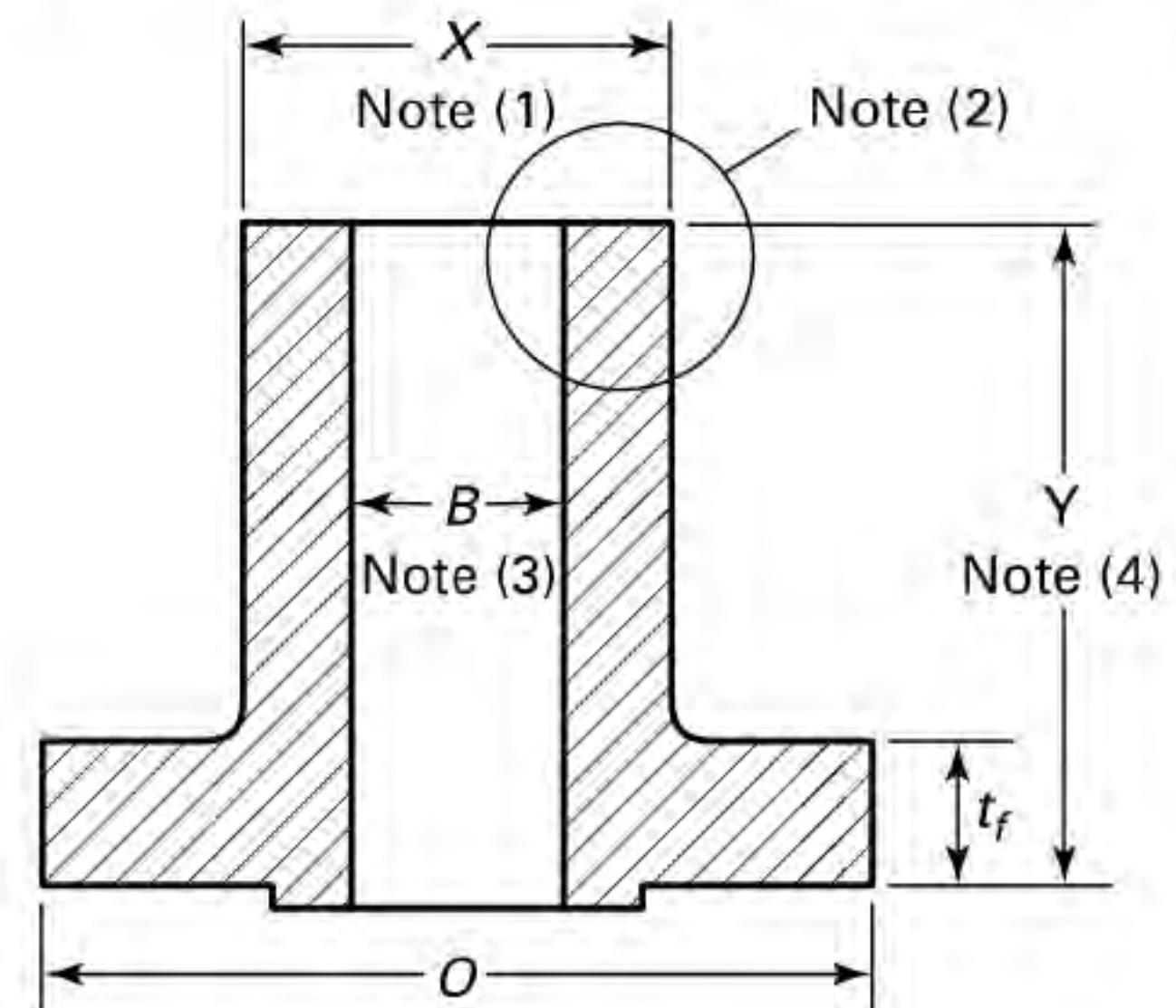
Figure 4 Straight Hub Welding Flanges
