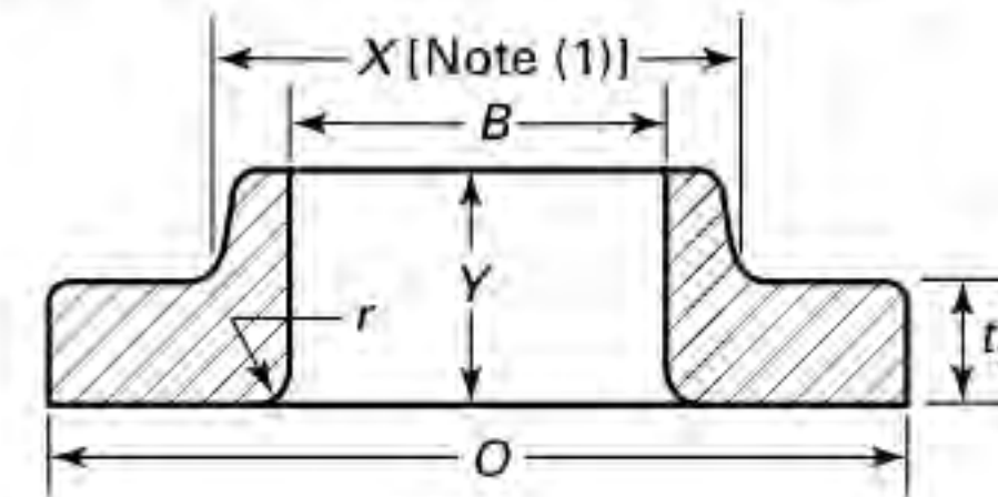
Lapped
