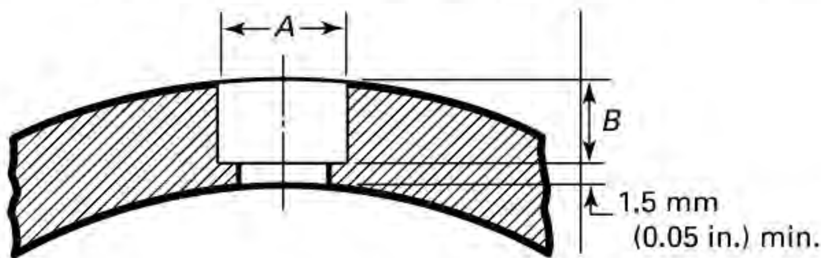
Figure 12 Socket Welding for Connections
