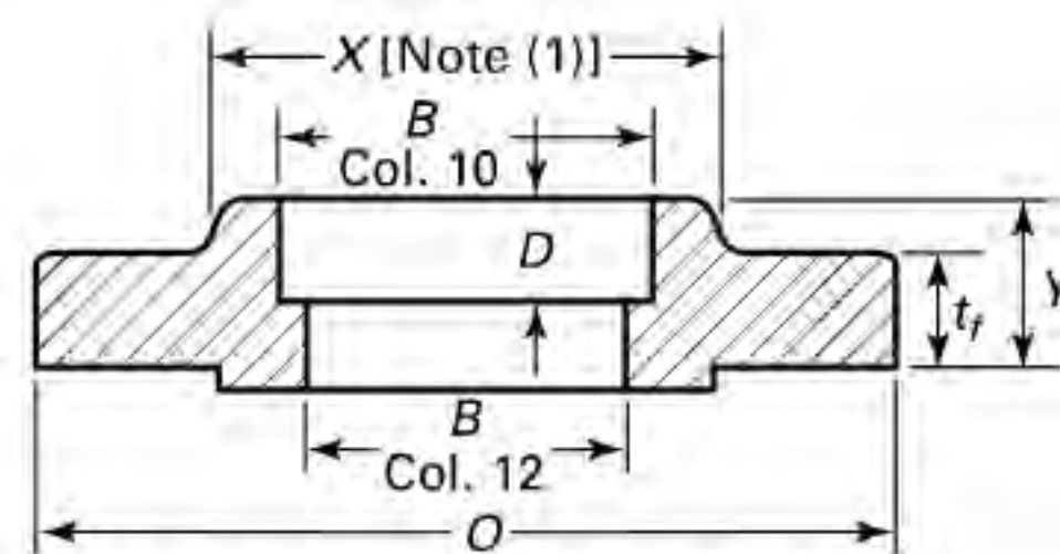
Socket Welding (NPS 1/2 to 2 1/2 Only)
