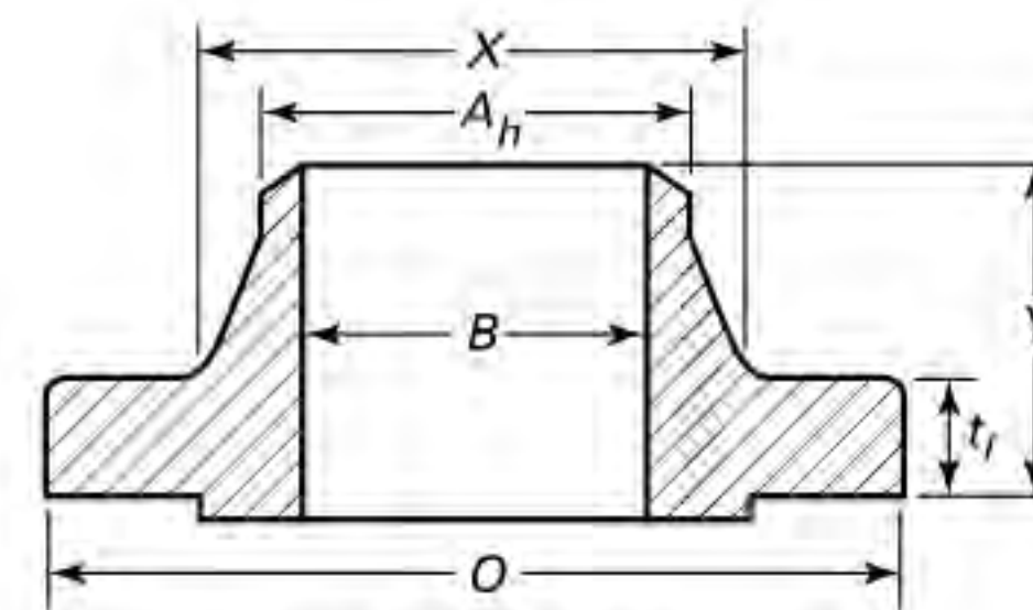
Welding Neck
