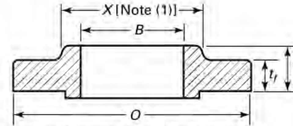
Slip-On Welding (NPS 1/2 to 2 1/2 Only)
