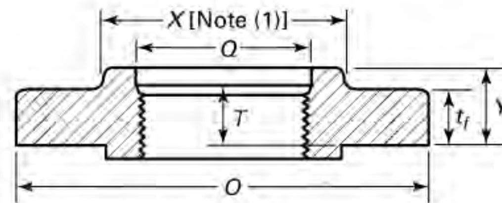
Threaded
