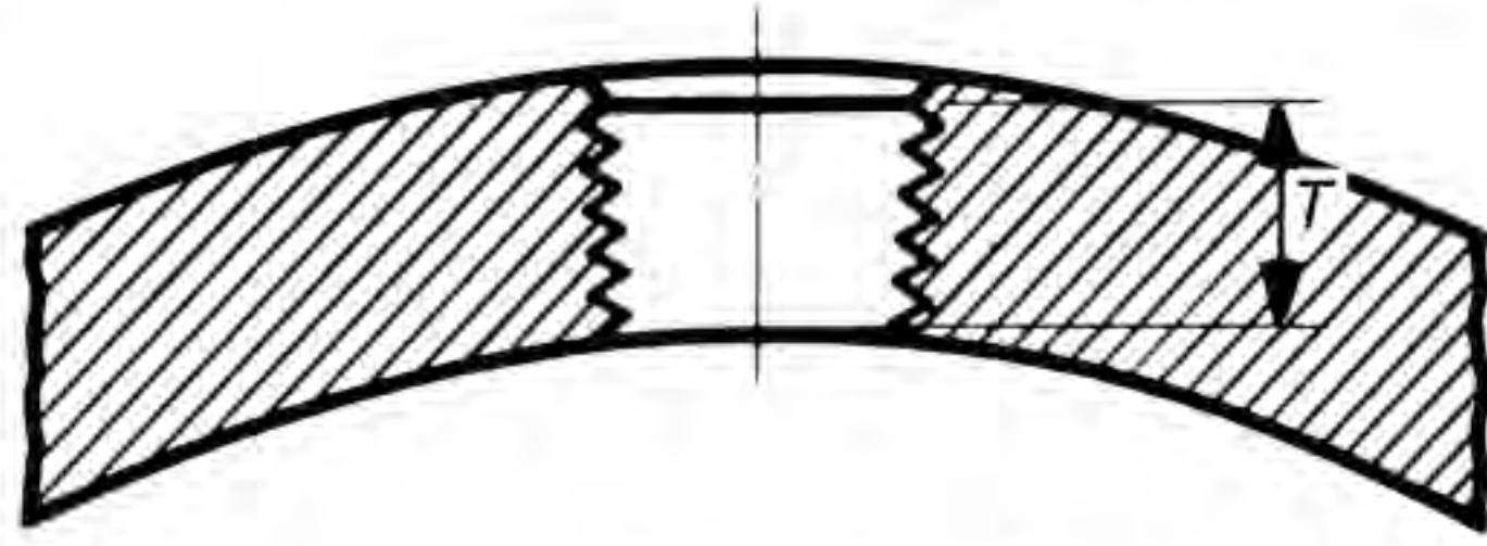
(20) Figure 11 Thread Length for Connection Tapping
