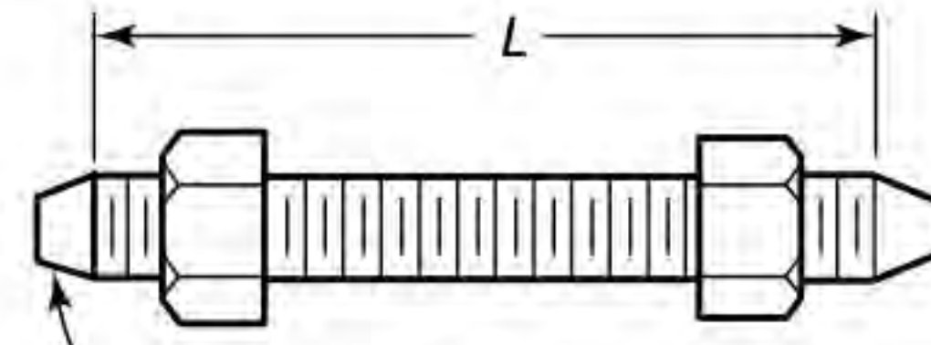
Stud Bolt With Nuts
