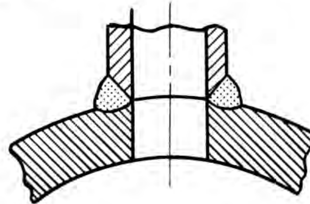
Figure 14 Butt Welding for Connections
