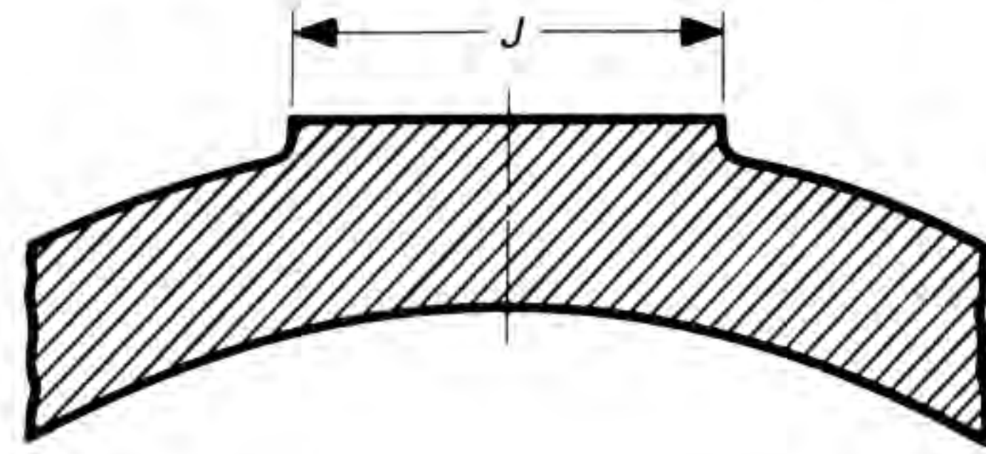
Figure 13 Bosses for Connections
