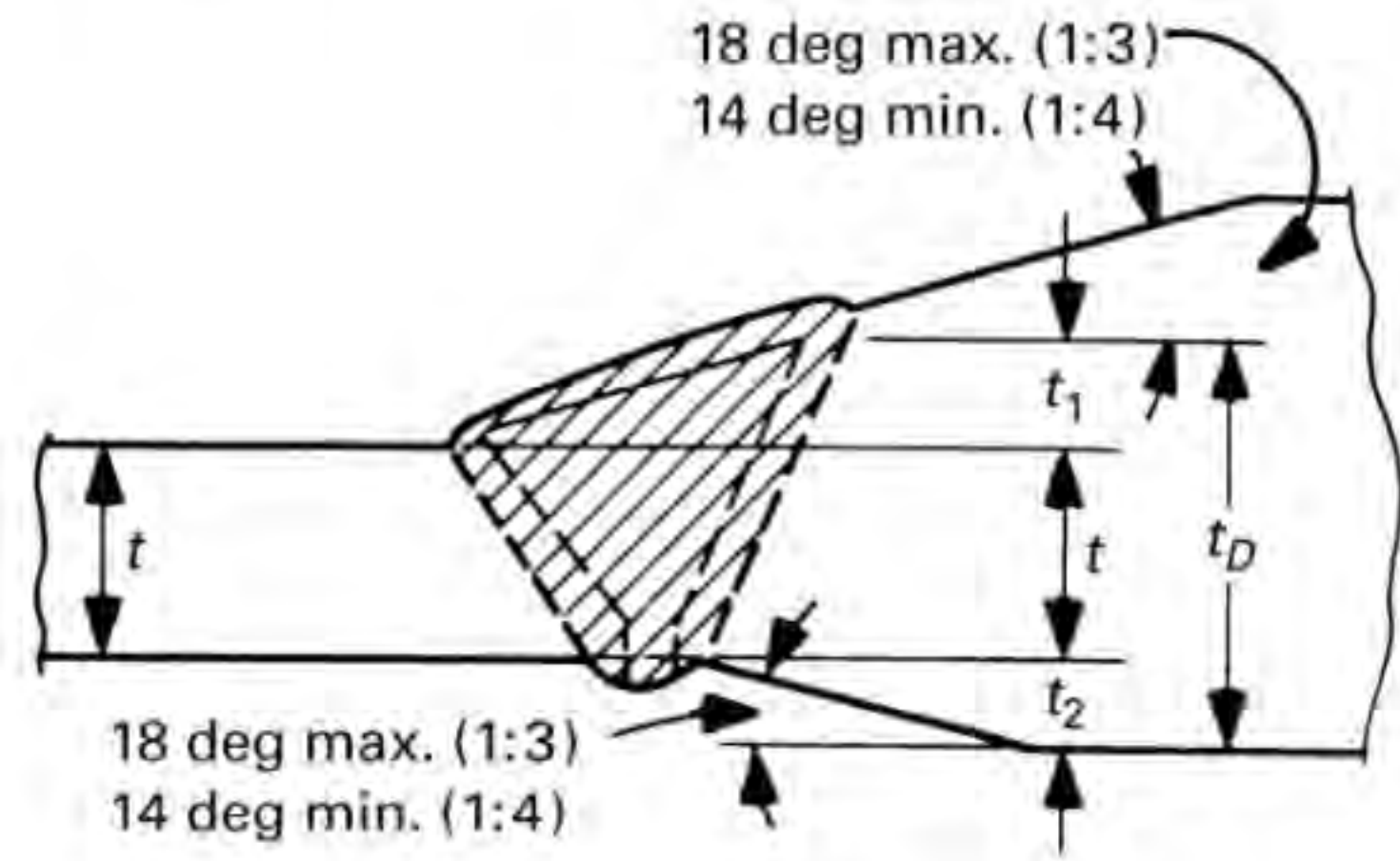
Figure 3 Bevel for Combined Thickness
