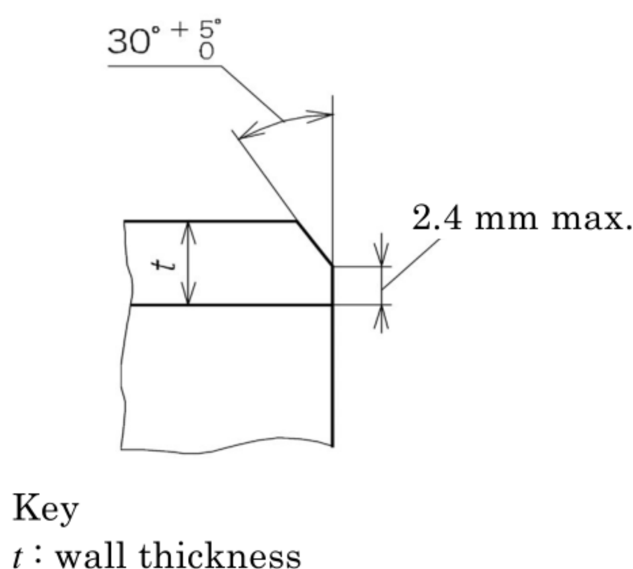
Figure 1 Shape of bevel end
