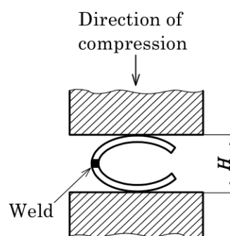
Figure 3 Flattening test (C-shaped test piece)
