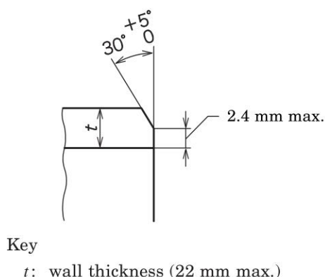
Figure 1 Shape of bevel end
